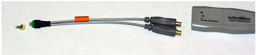
Figure 26 Recommended N5425A ZIF Probe Head for XAUI Testing
